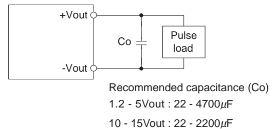
Fig.3.5 Connection for pulse load
