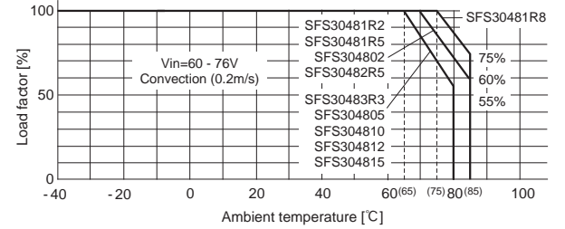
Fig.8.14 Derating curve (Convection)
