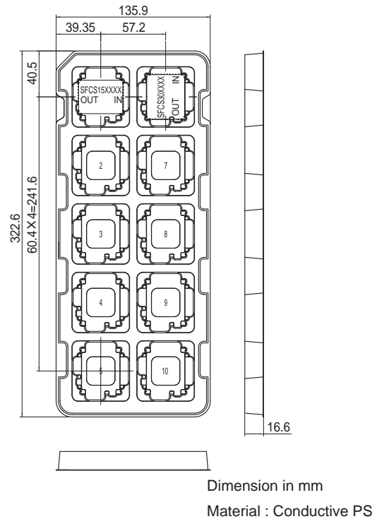
Fig.9.4 Delivery package information(SFCS15/SFCS30)
