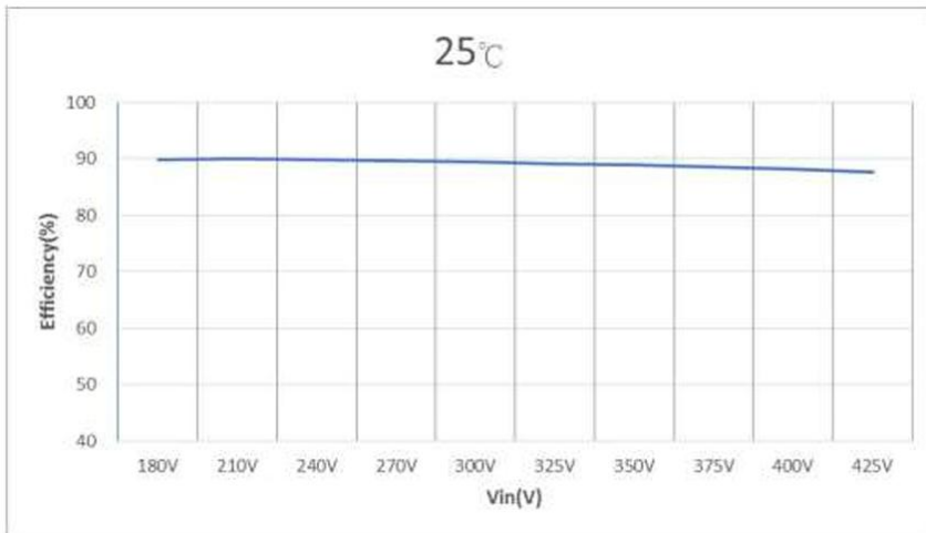
Figure 2 : Efficiency VS. Input Voltages at 100% rated power
