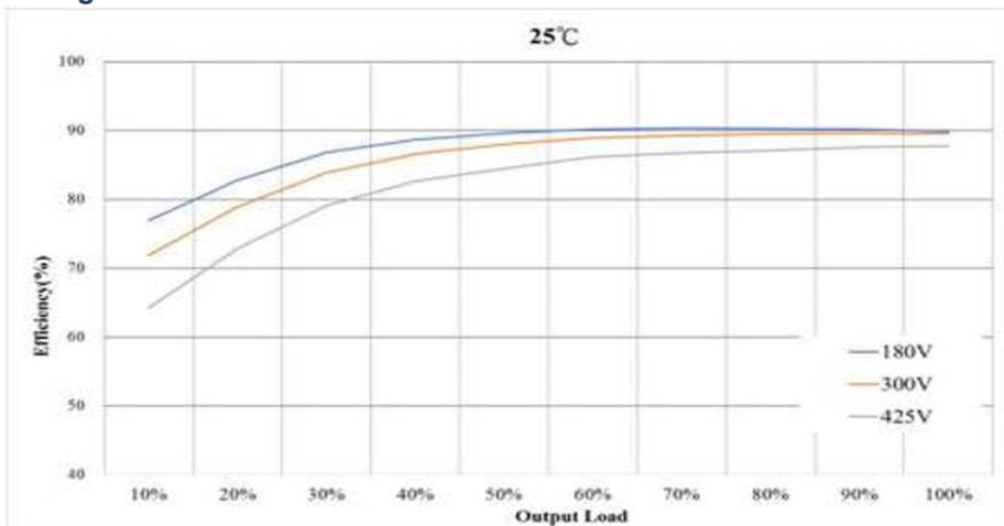
Figure 1 : Efficiency at Minimum, Nominal and Maximum Input Voltages VS. Output Load.
