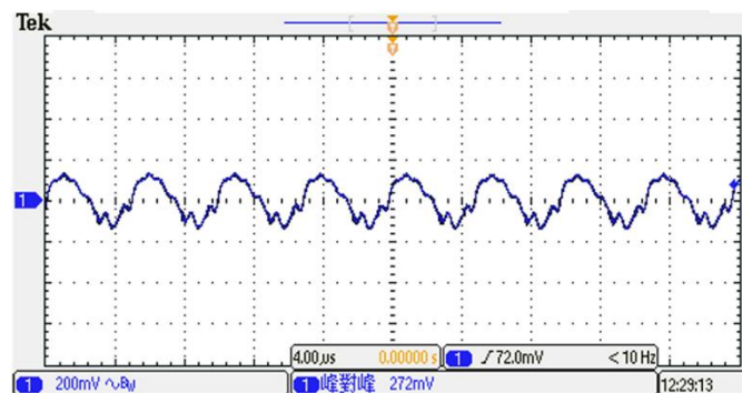
Figure 8 : Output Voltage Ripple & Noise at full load. ( V_{in} : Typical, With Output Capacitor to add 1µF MLCC)
