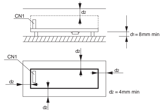
Fig.3.1 Installation method
