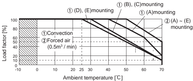
Fig.3.5 Ambient temperature derating curve (refer to Table 3.3)
