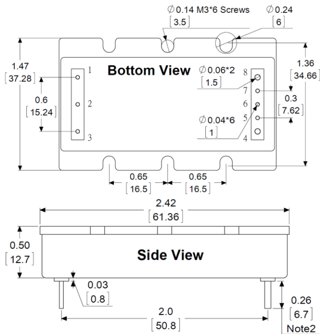
Shape – B (Base Plate with Vicor pinout)
