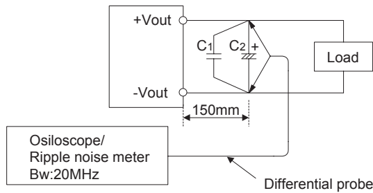
Fig.2.1 Measuring method of Ripple and Ripple Noise
