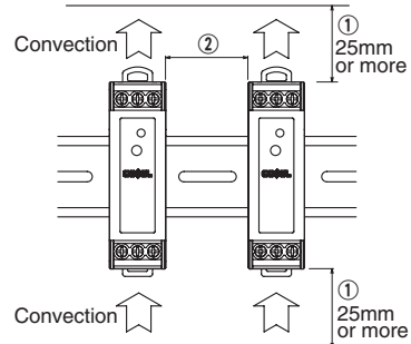
Fig.5.3 Installation clearance
