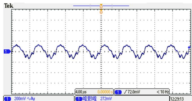
Figure 8 : Output Voltage Ripple & Noise at full load. ( V_{in} : Typical, With Output Capacitor to add 1μF MLCC)
