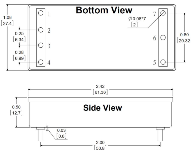
Shape – WB (Base Plate with DOSA pinout)
