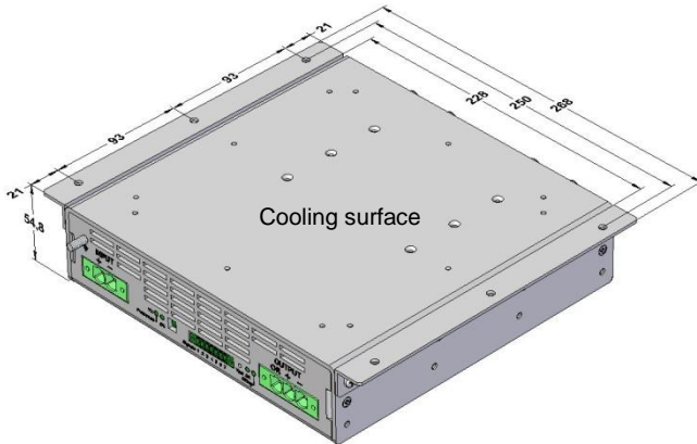
Conduction cooling version (Peso / weight 2.5kg)
