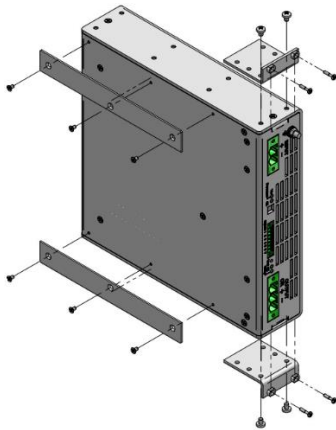
NP-9354 Rackmount tray
