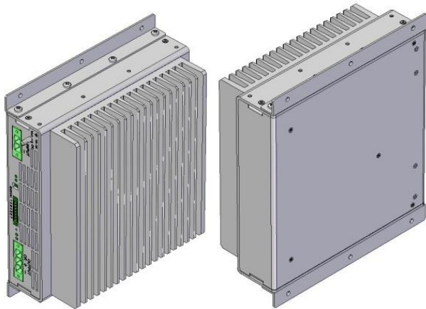
Conduction cooling version (Peso / weight 2.5kg)
