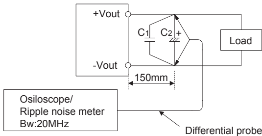
C1: Film capacitor 0.1 μF C2: Aluminum electrolytic capacitor 22 μF
