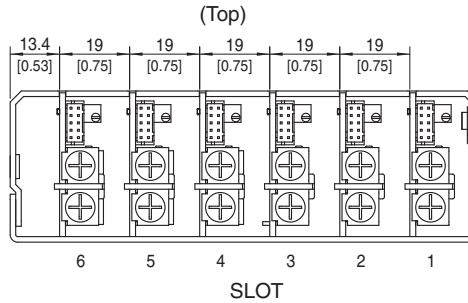
AME1200F Output side view
