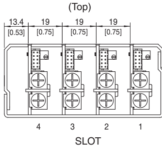
AME600F Output side view
